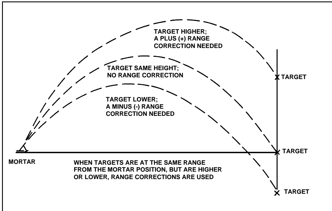
Figure 14-10. Altitude correction.
