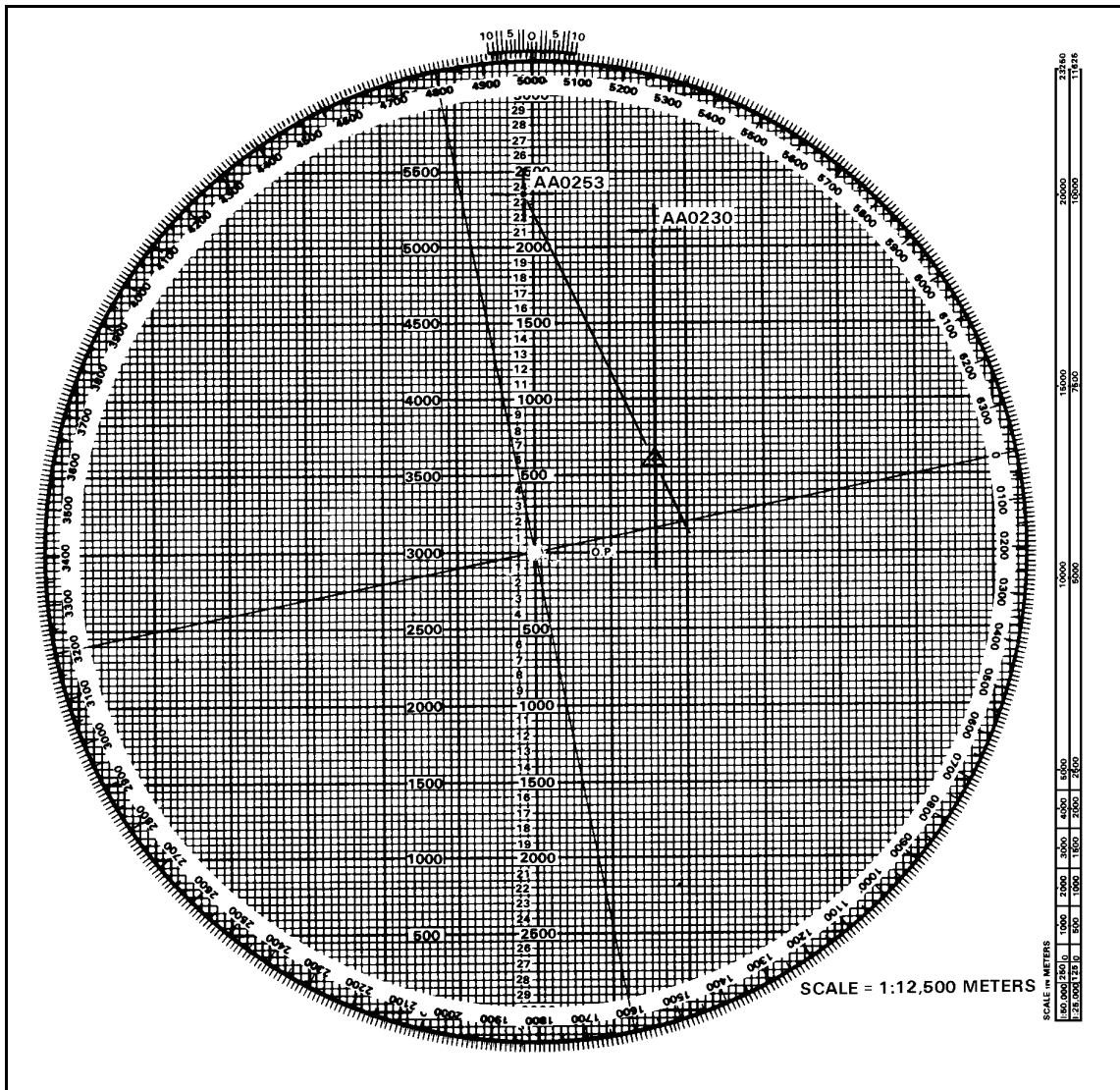
Figure 12-23. Resection.
